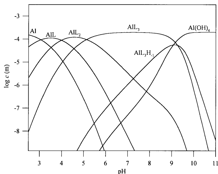
Fig. 2 Logarithmic distribution diagram of most important aluminium species in the presence of HL (aqueous 0.6 m NaCl, T = 25 °C, [Al]_0 = 2 \times 10^{-4} m , [HL]_0 = 10^{-3} m ; pK_s of amorphous Al(OH)_3 = -10.8 , pK_s of AlL_3 = 26.58 ).
