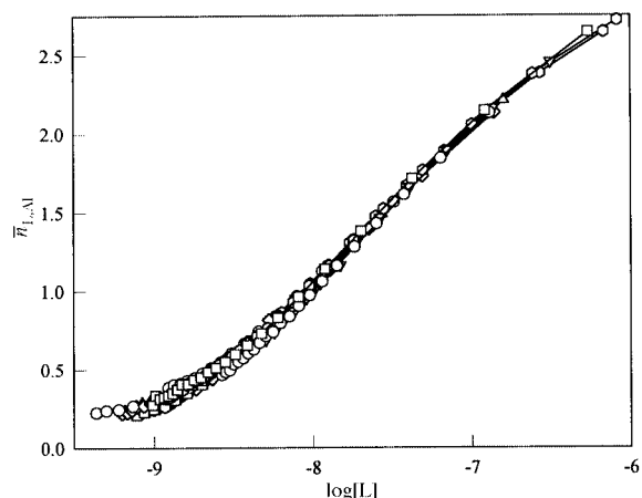
Fig. 1 Experimental data from the Al^{III} -HL system (25 °C) plotted as \bar{n}_{L,M} vs. \log [L] curves at various ligand and metal concentrations.
